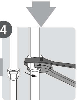
Connect the refrigerant pipes
