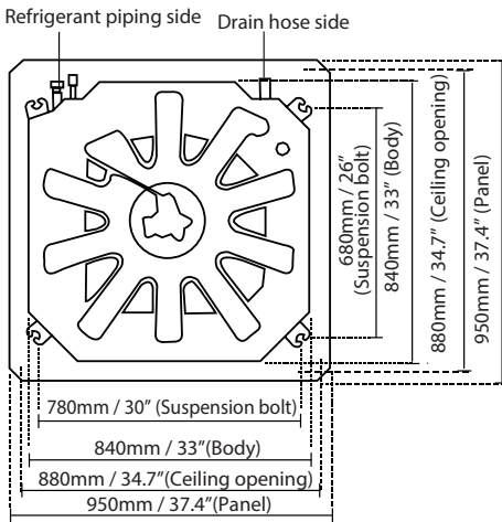
18-48K Super-Slim models ceiling hole size
